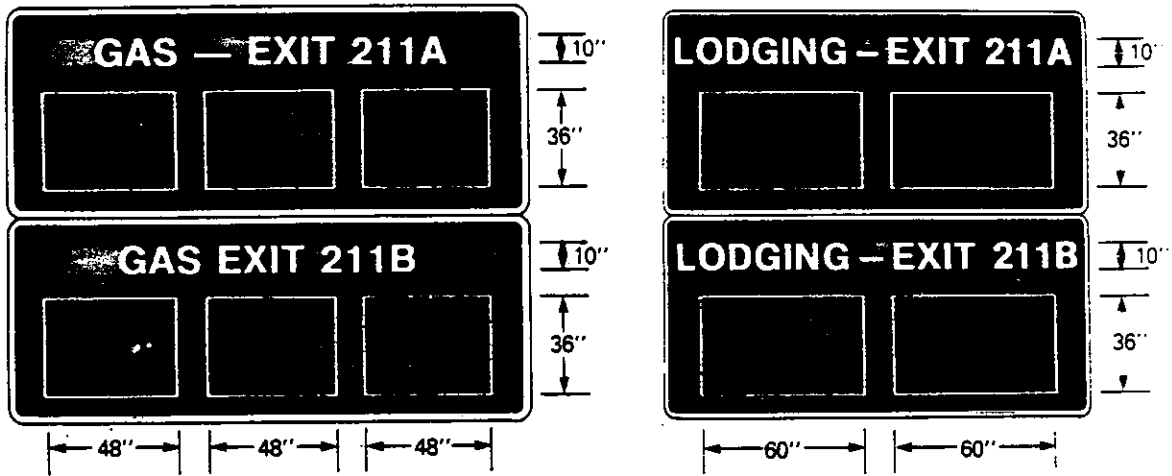
DOUBLE EXIT INTERCHANGE
